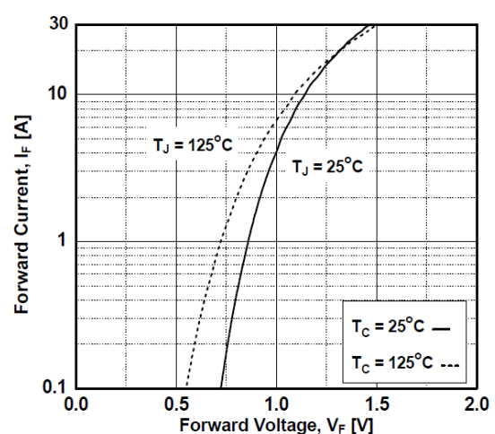
Figure 18. Forward Characteristics
