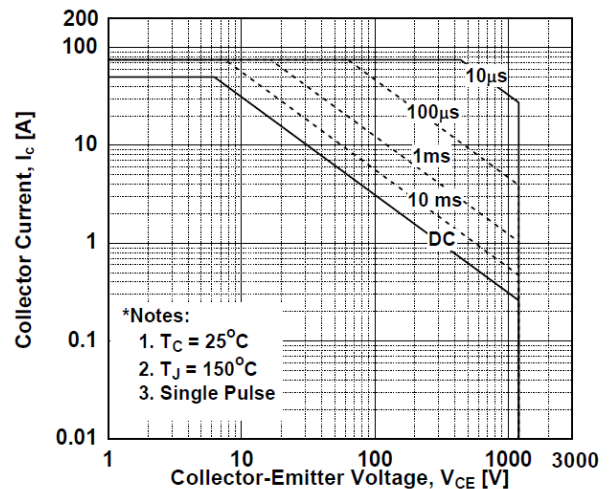
Figure 10. SOA Characteristics
